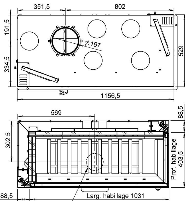
Raccordement air de combustion —
